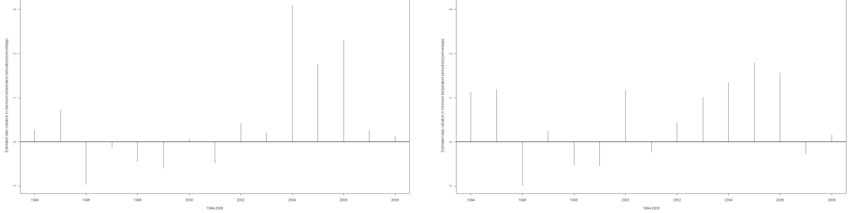
Figure 5: Estimated daily variation by year (annualized percentage) in maximum ( left ) and minimum ( right ) temperatures during the period 1994-2008
